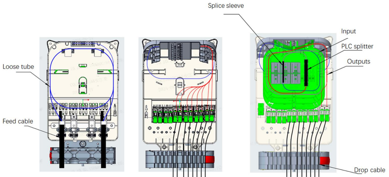
Figure 4 Splitter Routing
