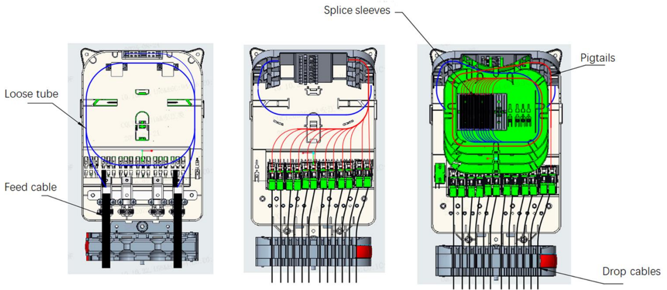
Figure 3 Splice Routing
