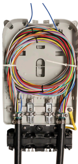
Cable entry and buffer tube storage
