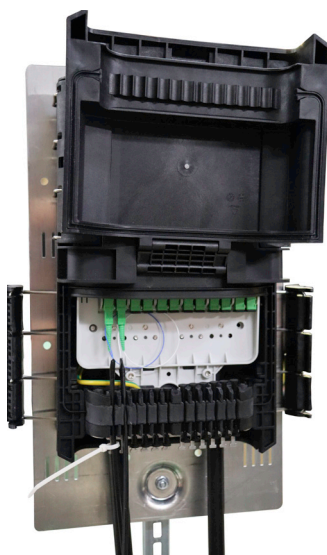
Drop cable entry
