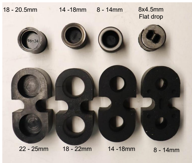
Figure 4 Grommets included with FODC-C2
