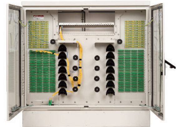
OHC-864 Double door front and back form factor, pad mount only
