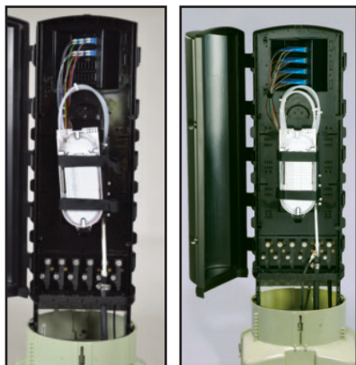
CFDP210-EL12L/A (left) AND CFDP210-EL24F/A (right) FTTCS PEDESTALS WITH FIBER SPLICE COMPARTMENT AND BULKHEAD ADAPTERS
