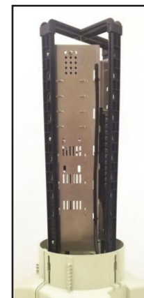
CP210-CTFT/ATT FOR MST, COPPER TERMINAL, AND COPPER SPLICE (views of 3-sided backboard)
