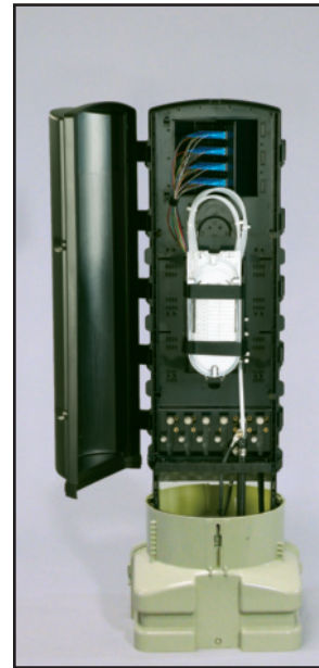
CFDP210EVL24F/A Fiber to the Cell Site Pedestal (Handhole Mount)
