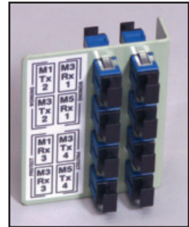
80-002665-F Eight Position Bulkhead Plate for Ring Configurations
