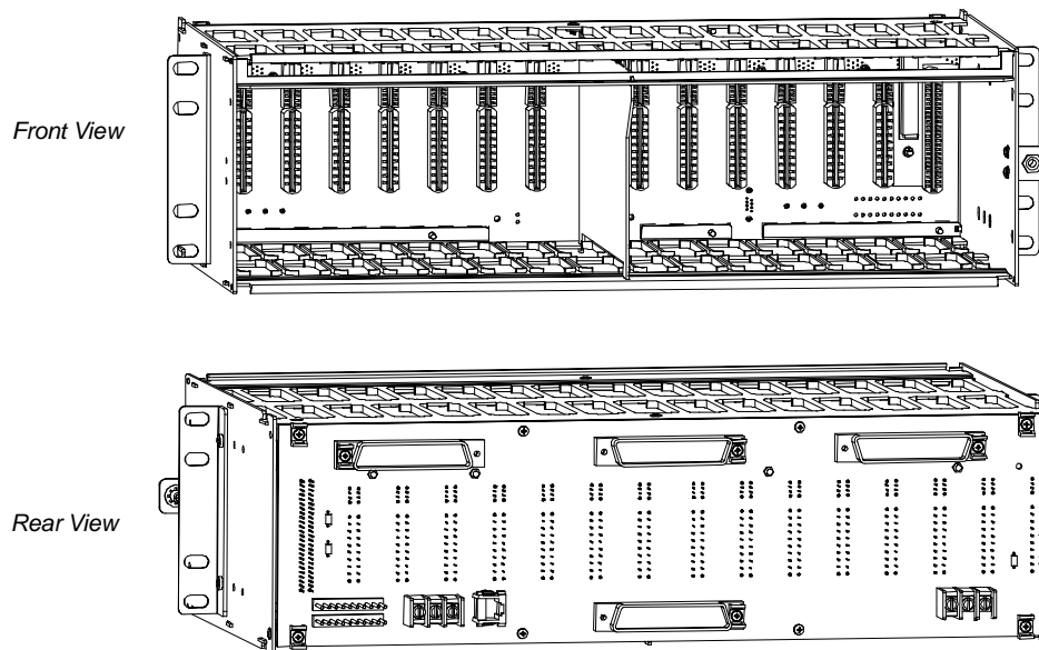
Figure 1. HVDL315 COT Shelf
