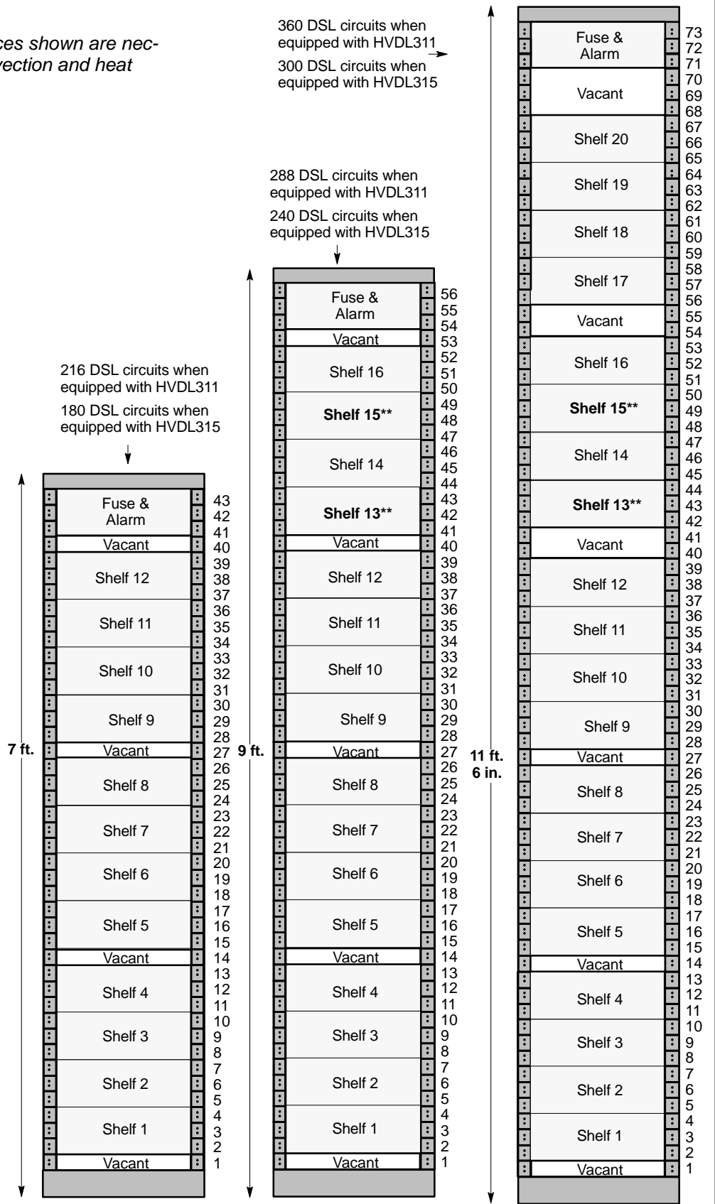
Figure 3. Fully Equipped Rack Profiles with HVD31X Shelves and DDL3XX Cards
