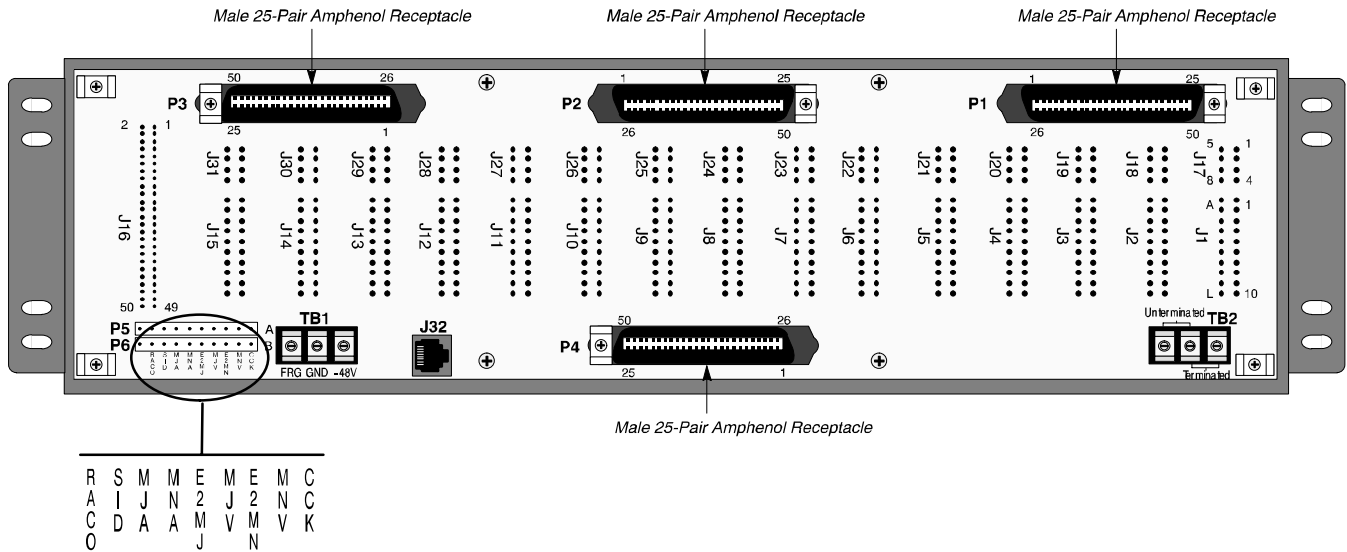
Figure 6. HVDL315 Rear View
