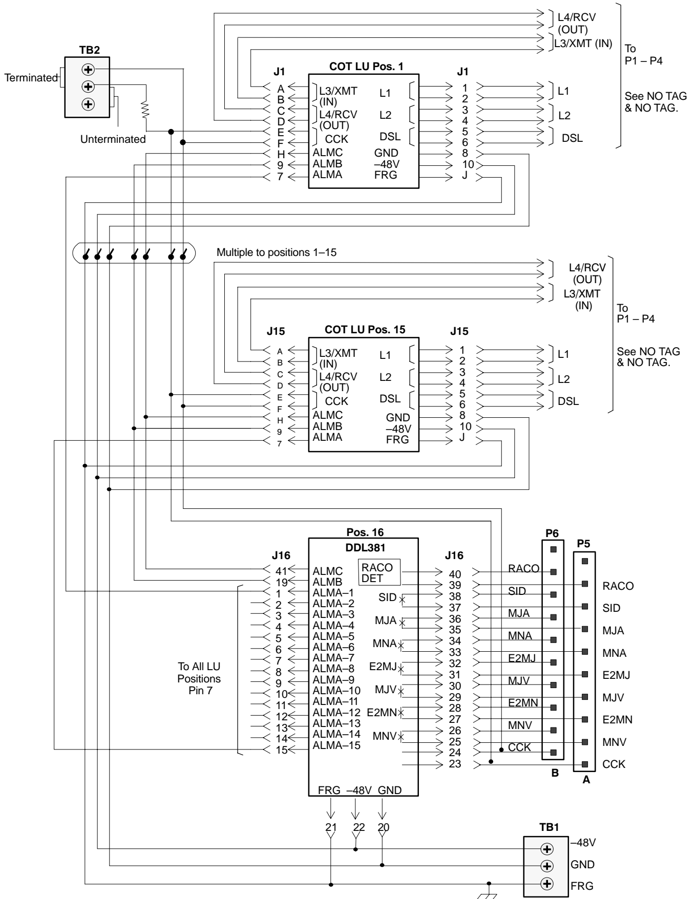
Figure 8. HVDL315 Shelf Wiring Diagram
