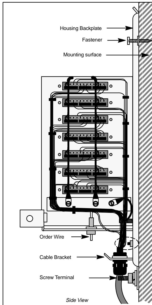
Figure 6. Rotated Module Housing Exposing Module Connector Pins And Wiring
