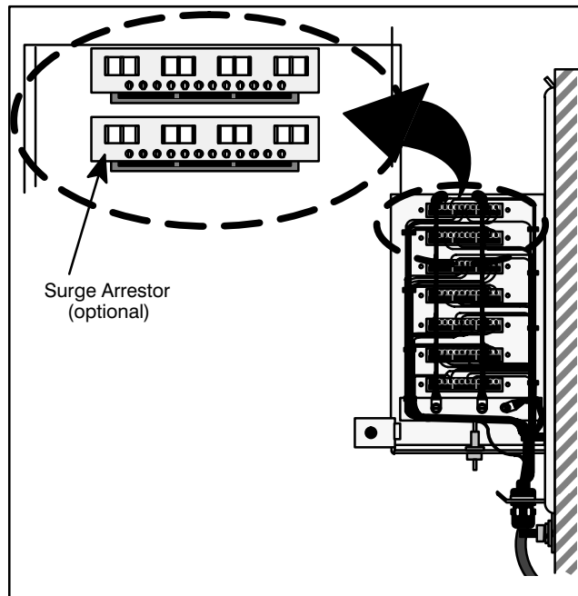
Figure 5. Optional CiSA-4 Surge Arrester Assembly Installed Over Pins
