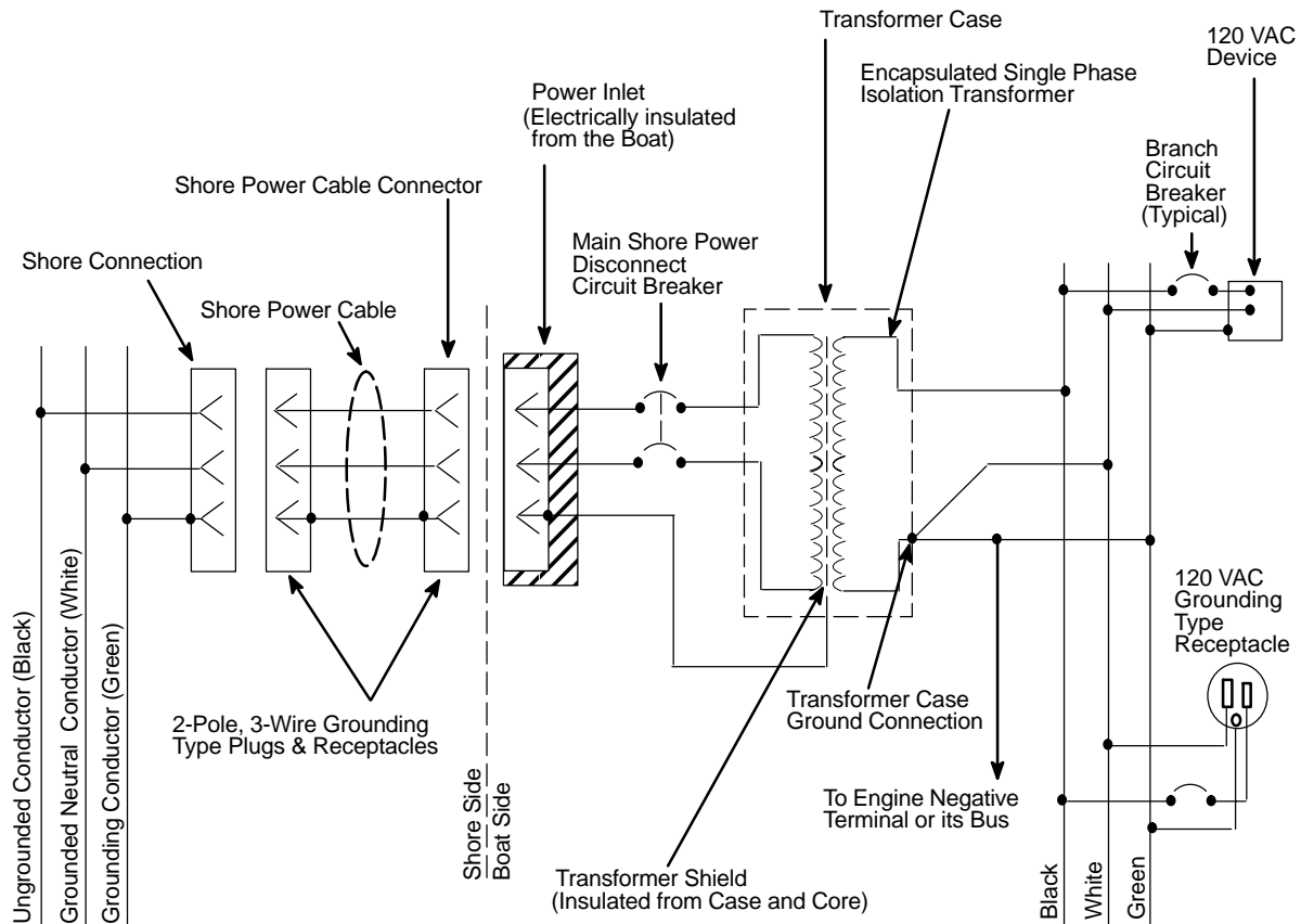
Figure 2. Electrical Diagram – Method 1 (see Figure 4 for Wiring Connections)
