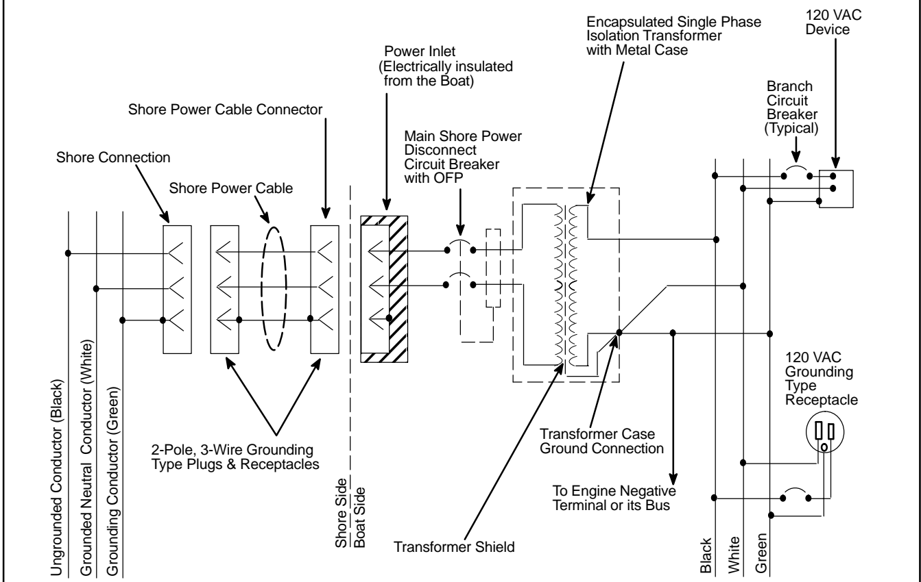
Figure 3. Electrical Diagram – Method 2 (see Figure 5 for Wiring Connections)
