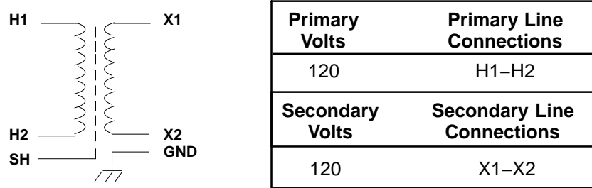
Figure 1. Schematic and Connections
