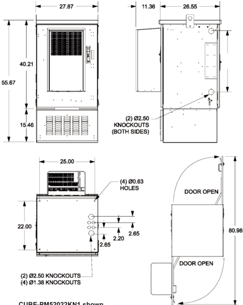
CUBE-PM52022KN1 shown
