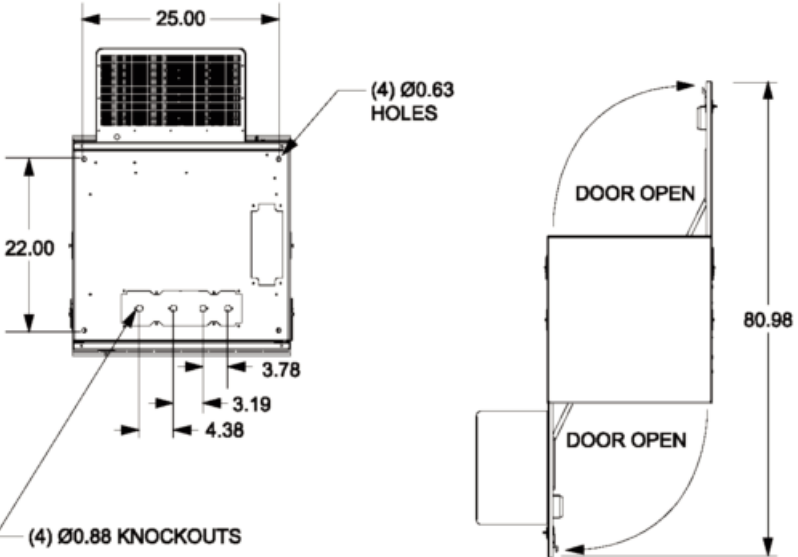
CUBE-PM53012LN1 shown
