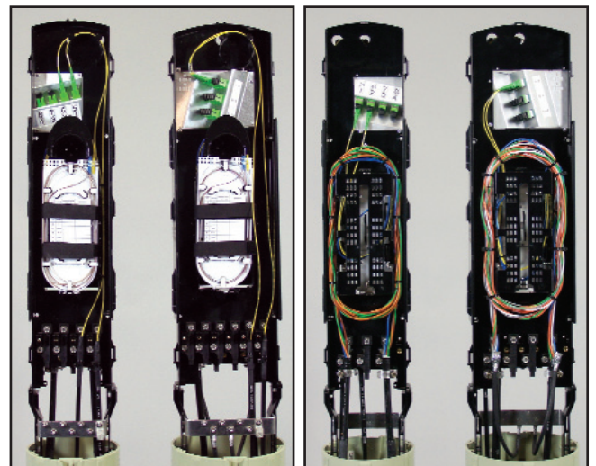
Central Office Side of Fiber Organizers
