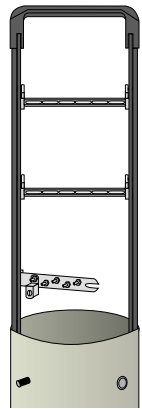
"S" BRACKET FOR BD2, BD3 & BD4
